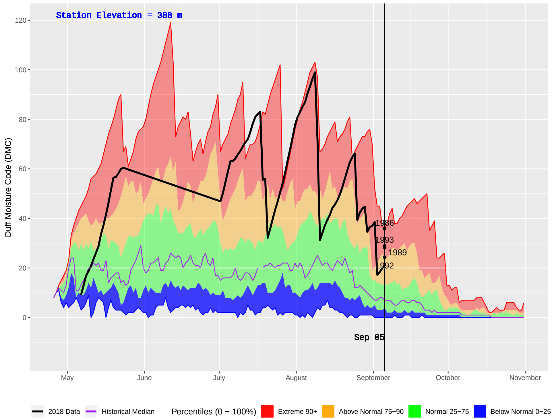
BELL-IRVING (432) : Historical (1986–2016) and Current (2018) Daily Duff Moisture Code (DMC)
