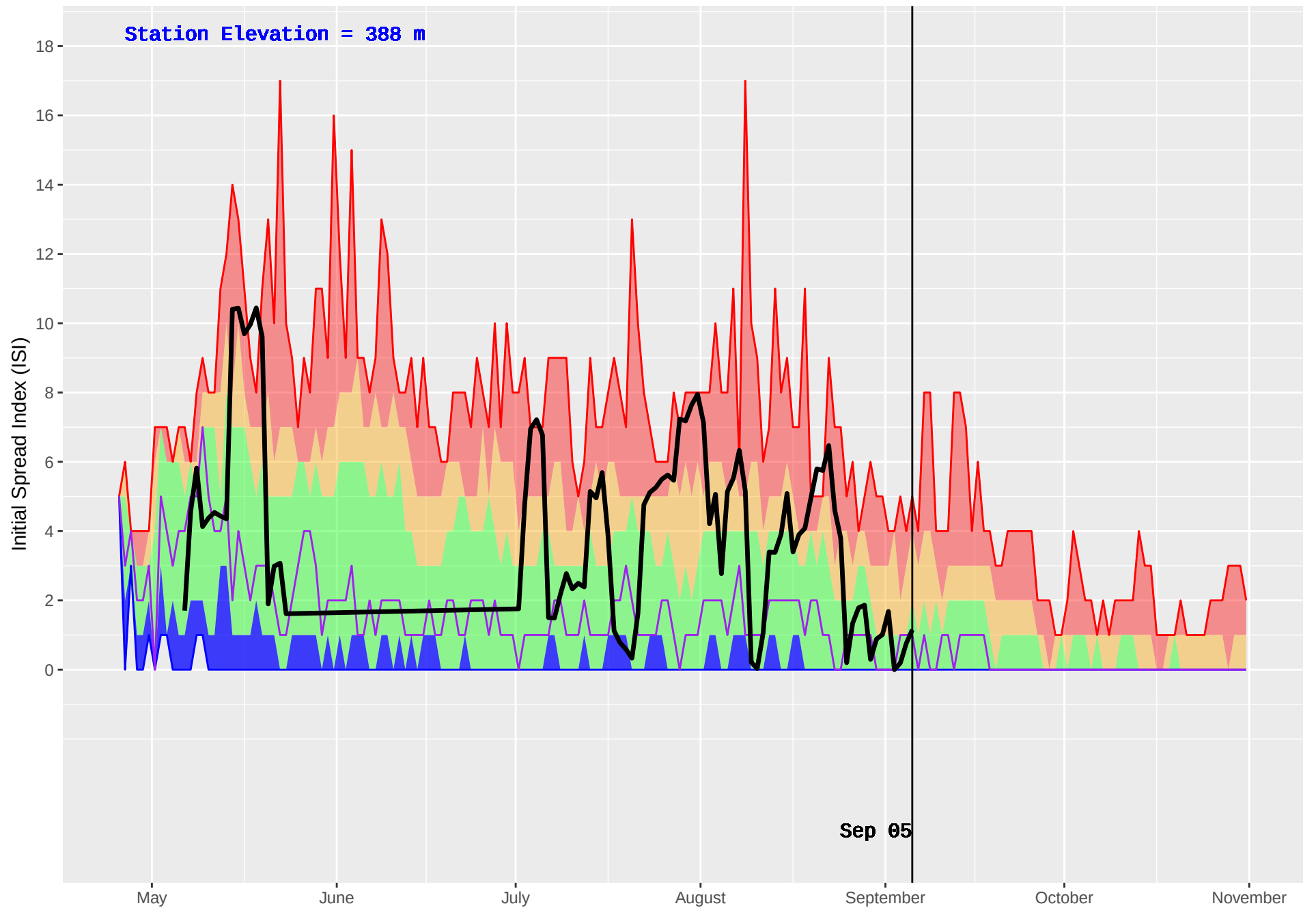
BELL-IRVING (432) : Historical (1986–2016) and Current (2018) Daily Initial Spread Index (ISI)
